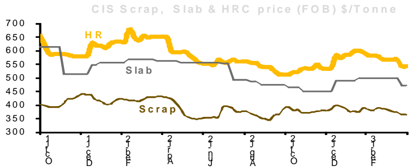
Figure 3: Black Sea Export Scrap, Slab & HRC price ($/Tonne)
